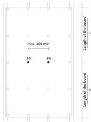
Figure 2: Combination of 2 fixed points
