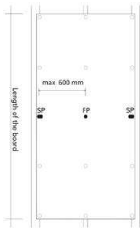
Figure 1: Combination fixed point and slotted points
