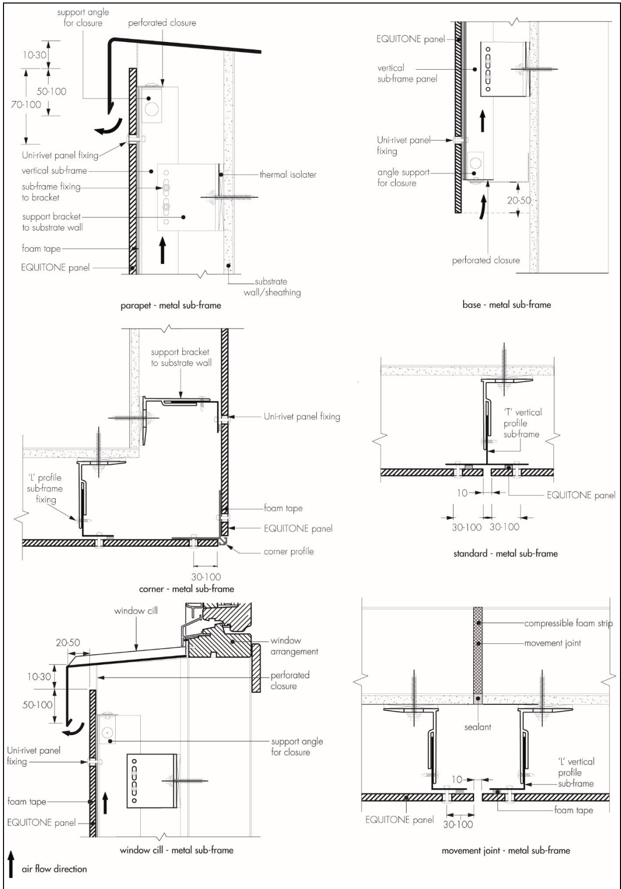
Figure 1 Typical installation details
