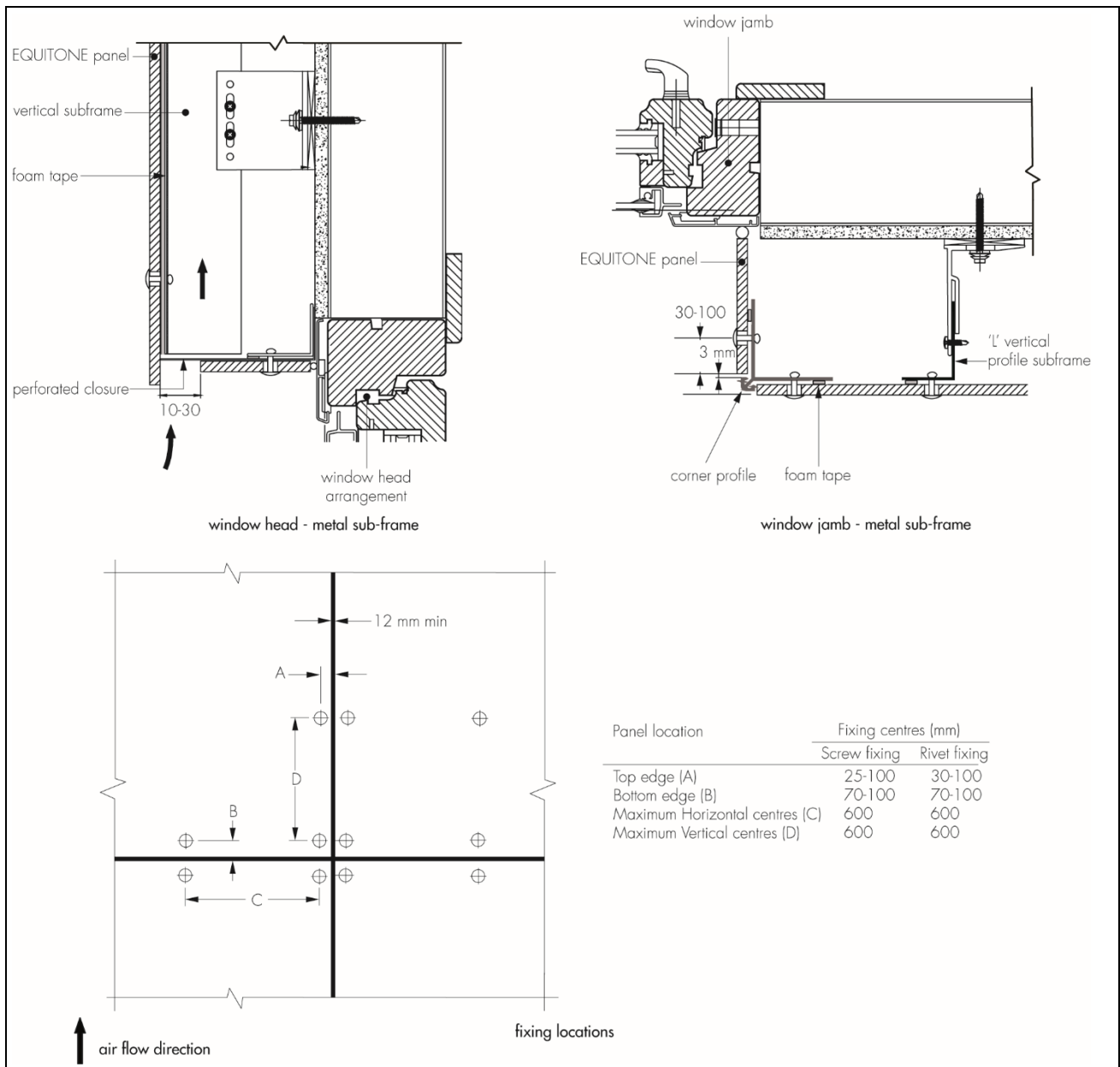
Figure 1 Typical installation details (continued)
